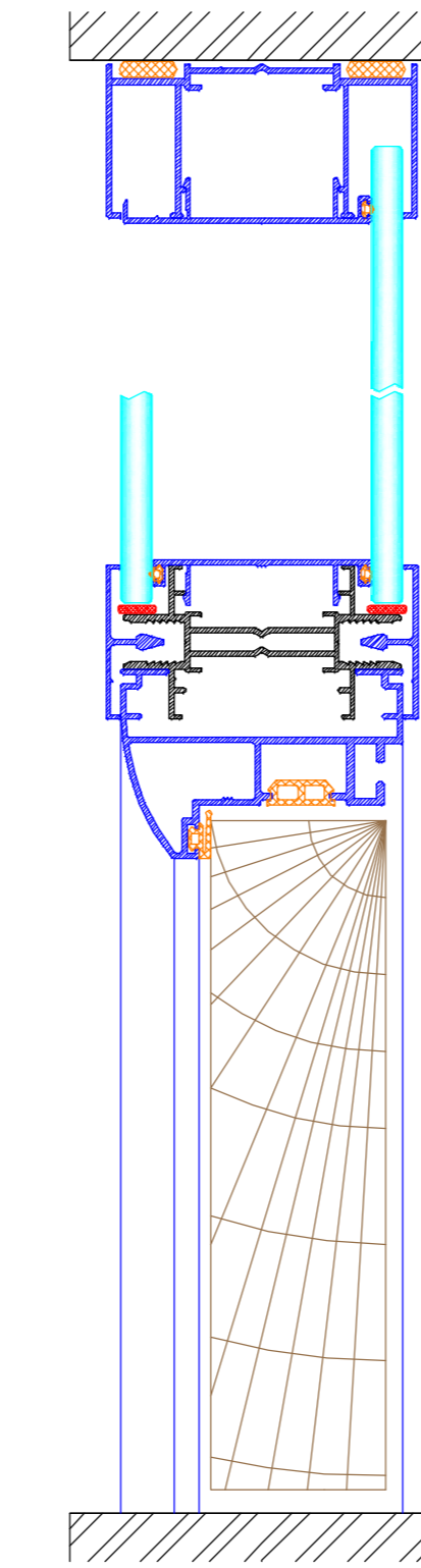
Porte Bois Standard Imposte Vitrée Standard Wooden Door with Glazed Impost
